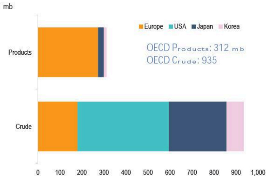
Figure 1: OECD SPR inventory
